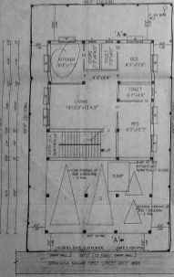
SITE PLAN/STILT AND GROUND FLOOR PLAN
